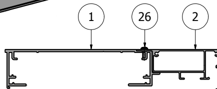
TOP CROSS-SECTION
