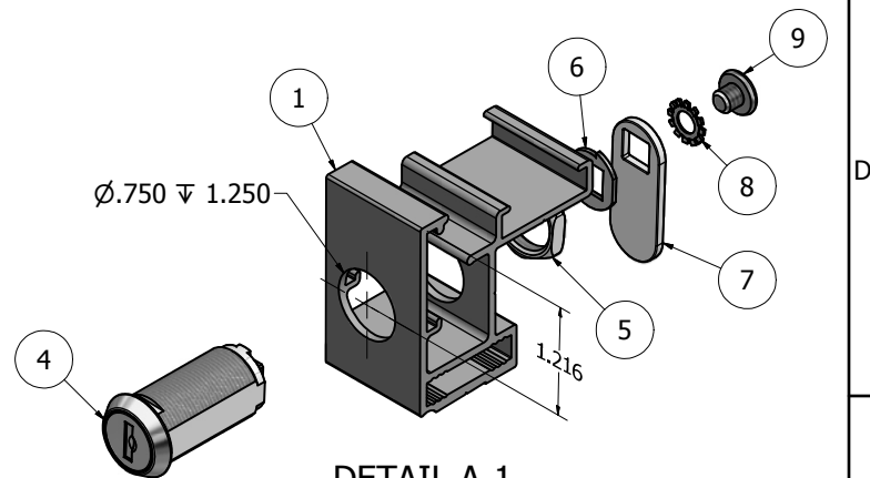
DETAIL A-1
